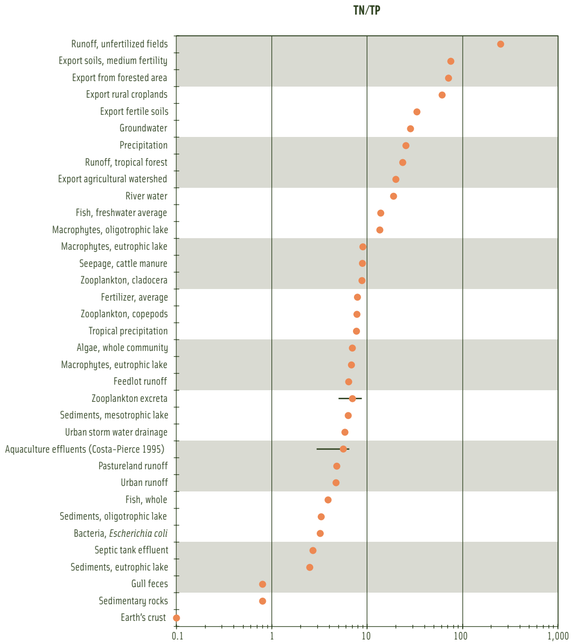
Figure 8. Total nitrogen/total phosphorus (TN/TP) ratios for various pollutants, and excreta and mass ratios of some aquatic organisms. To convert to molar ratios, multiply by 2.21. (Selected from Downing and McCauley 1992.)
