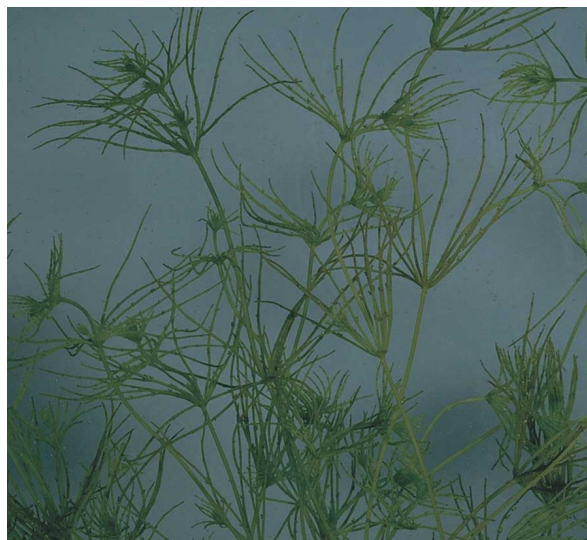
Figure 37. Macrophytic algae
