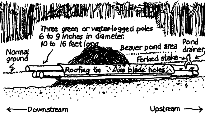
Three-log drain.
