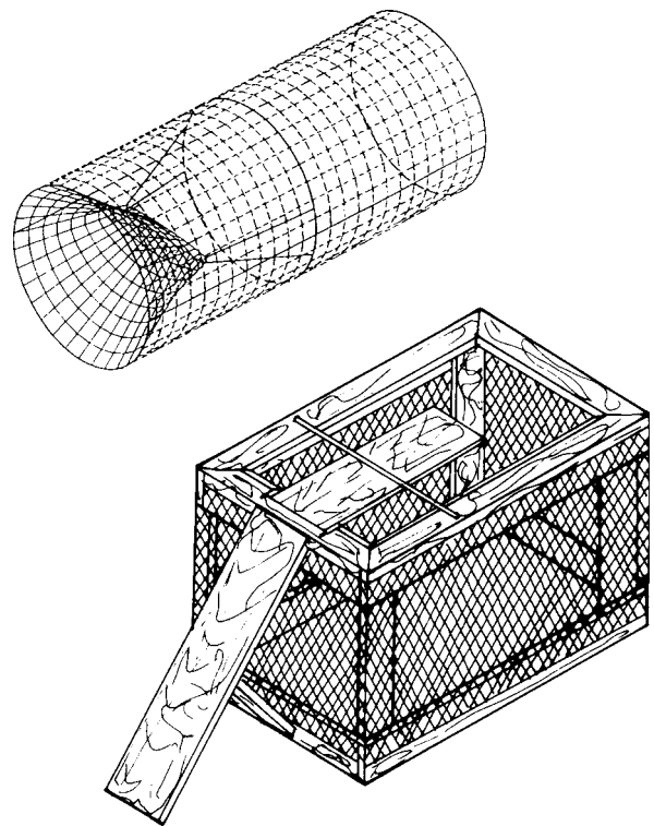
Figure 24. Turtle Trap Designs
